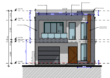
FRONT (North) ELEVATION
