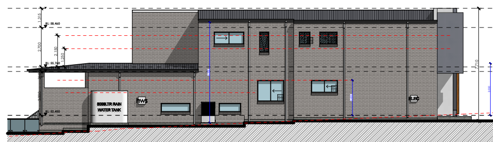
SIDE (East) ELEVATION
