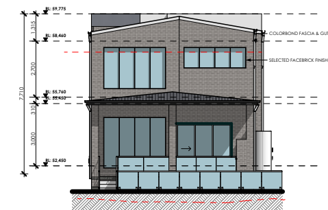
REAR (South) ELEVATION
